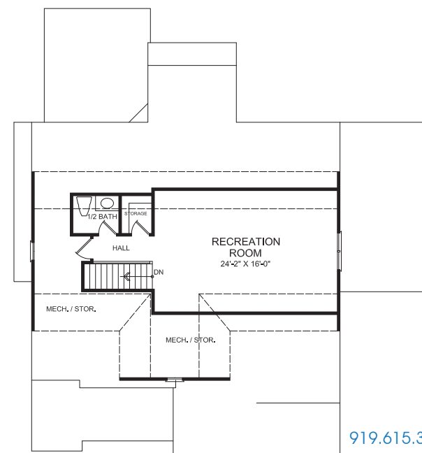
THIRD FLOOR
